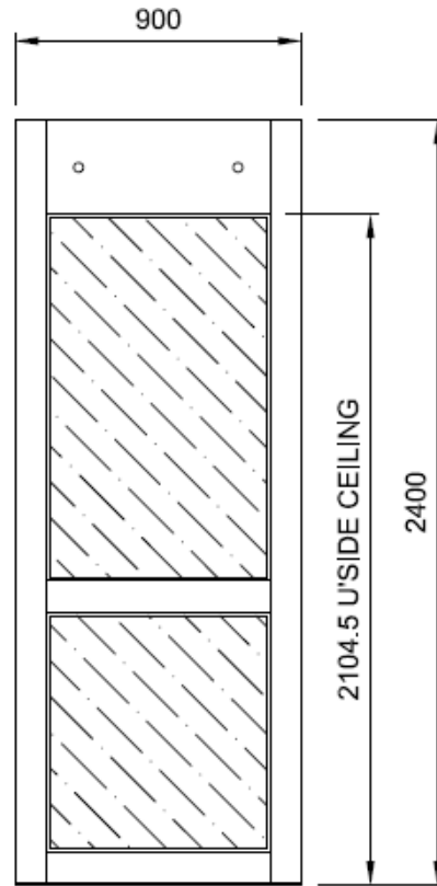
SIDE ELEVATION
